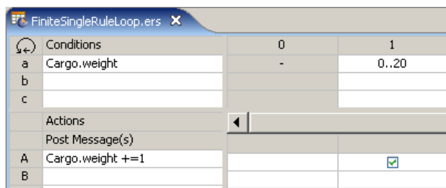
Figure 124: Example of a Finite Single-Rule Loop
