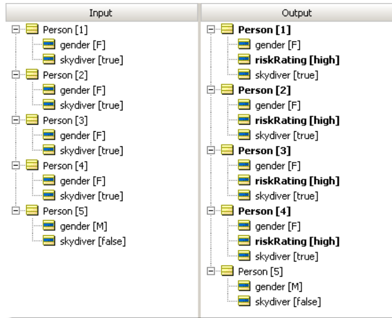
Figure 172: Ruletest
