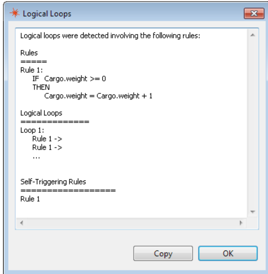
Figure 130: A Single-Rule Loop Detected by the Check for Logical Loops Tool
