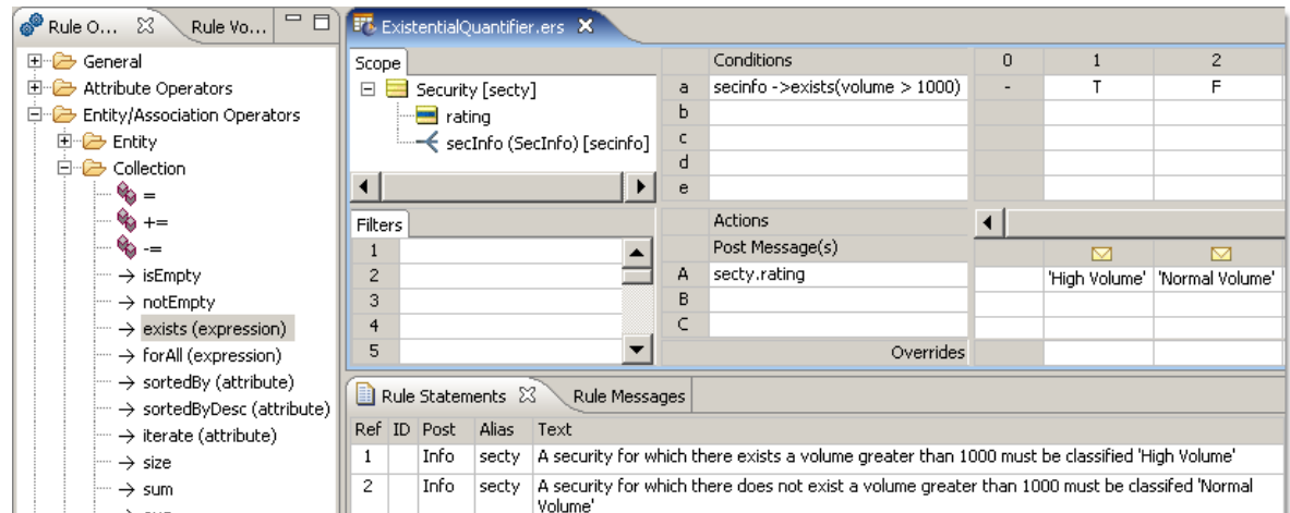
Figure 94: Rulesheet with Existential Quantifier ("exists") Condition
