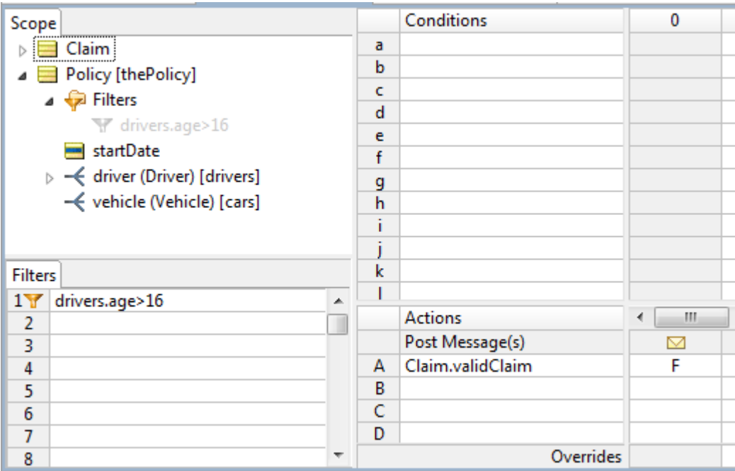
Figure 154: Rulesheet for Precondition
