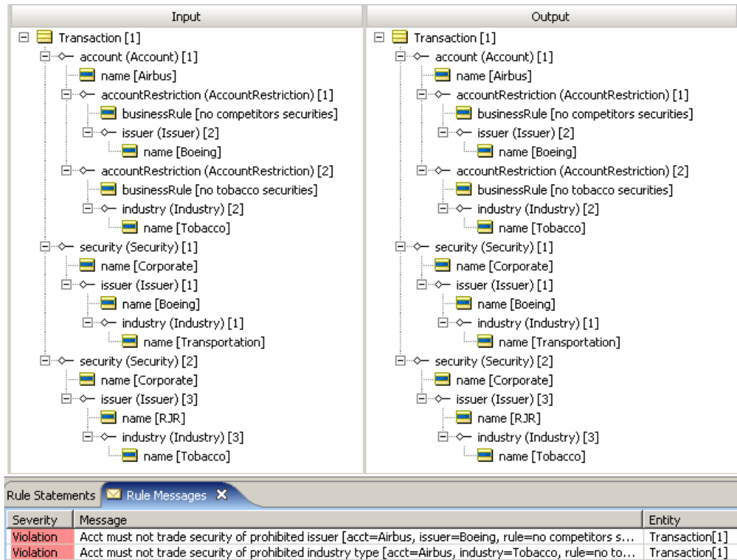
Figure 177: Ruletest
