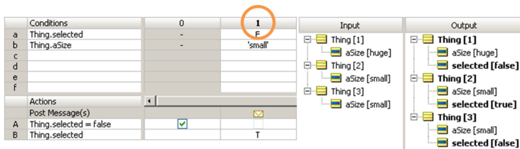
Figure 140: Rulesheet and Ruletest, threshold condition added, CaPT enabled
