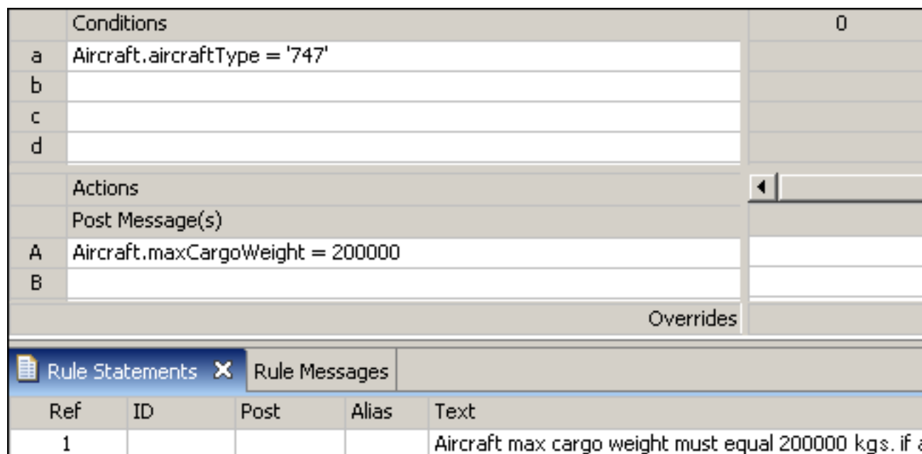
Figure 64: Rulesheet Using a Conditional Rule
