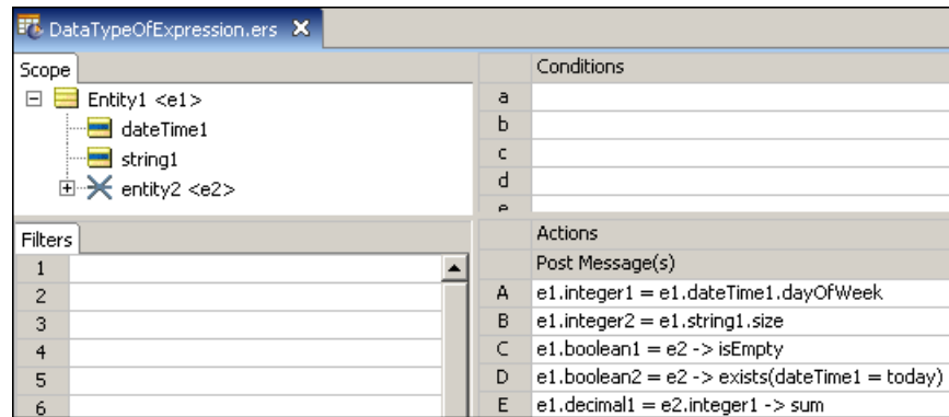
Figure 106: Examples of Expression Datatypes
