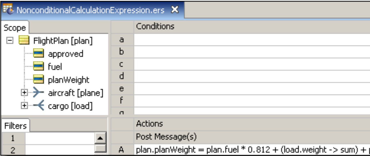
Figure 112: A Calculation in a Nonconditional Expression
