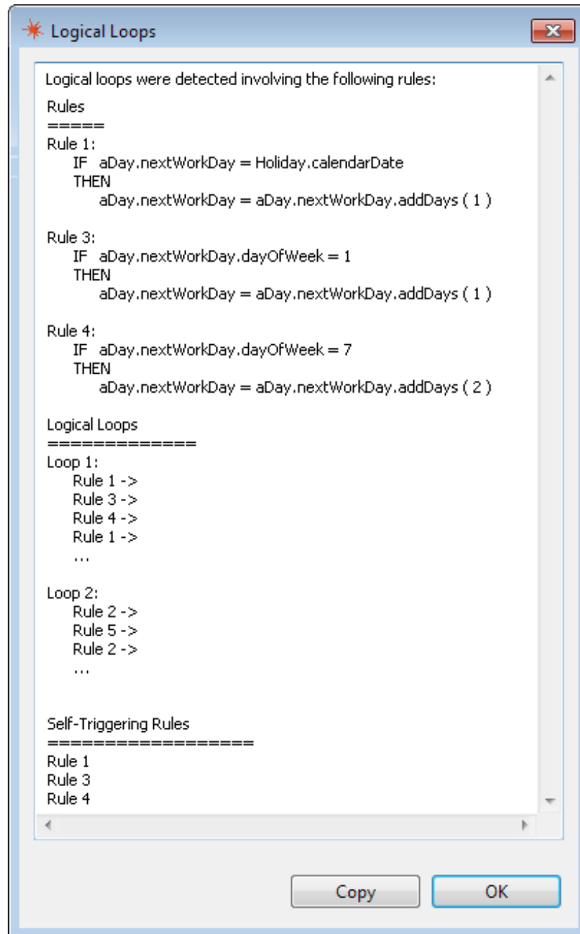
Figure 135: Results of Logical Loop Check
