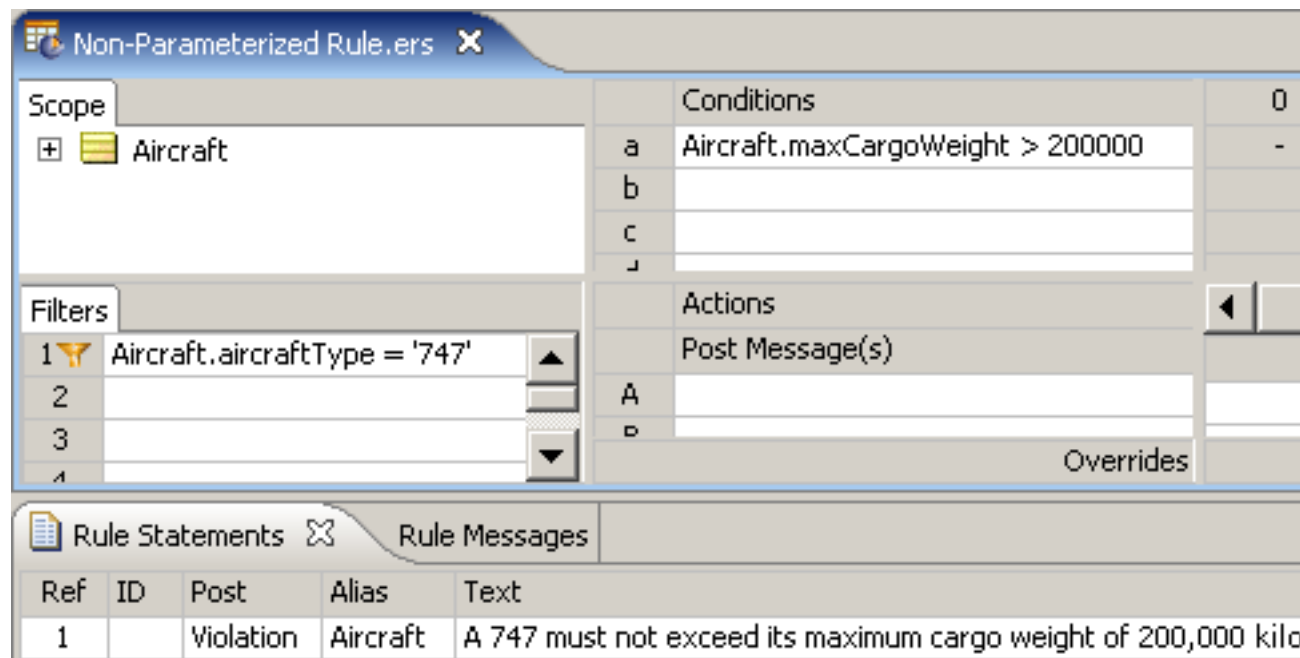
Figure 173: Non-Parameterized Rule
