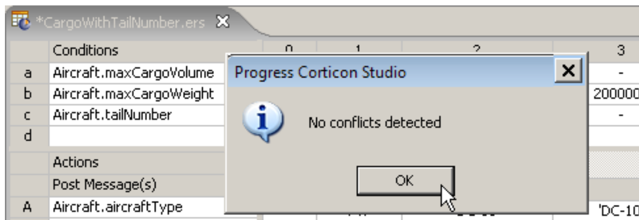
Figure 221: Proof that no New Conflicts have been Introduced by the Completeness Check
