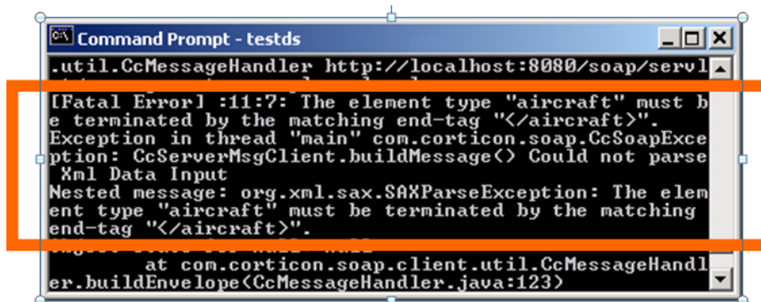
Figure 241: Server Window Message Highlighting Incorrect SOAP Request Structure
