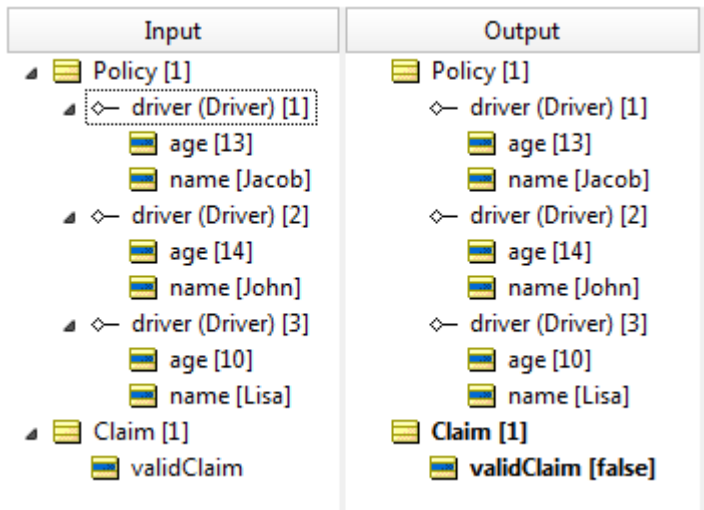
Figure 155: Ruletest for Precondition
