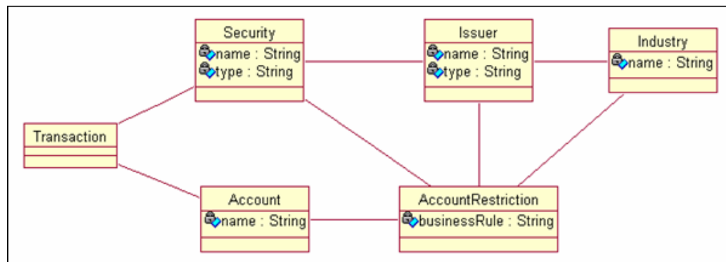
Figure 175: UML Class Diagram of Sample Vocabulary
