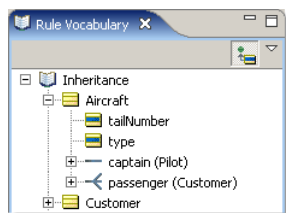
Figure 32: Vocabulary with Inheritance Properties Hidden
