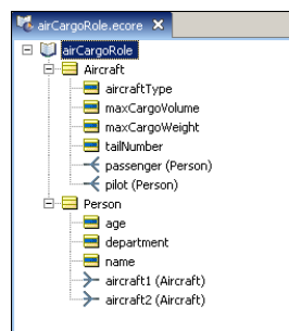
Figure 56: Vocabulary with Roles
