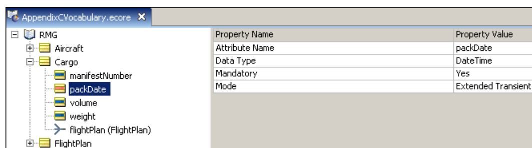
Figure 245: Vocabulary Editor Showing an Extended Transient Attribute
