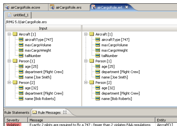
Figure 58: Ruletest with no Person entities in Pilot role
