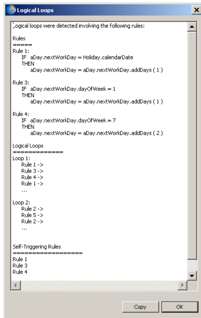
Figure 130: Results of Logical Loop Check
