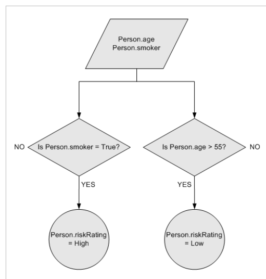
Figure 185: Flowchart with 2 Rules
