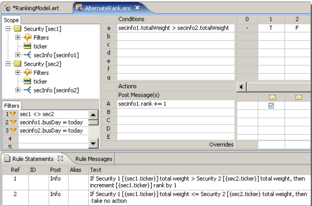
Figure 82: Rulesheet with Alternate Rank Determination Rules
