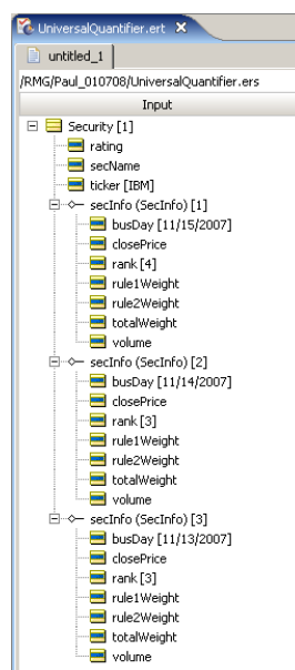
Figure 87: Ruletest for Testing “for all” Condition Rules
