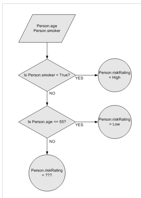
Figure 186: Flowchart with 2 Dependent Rules
