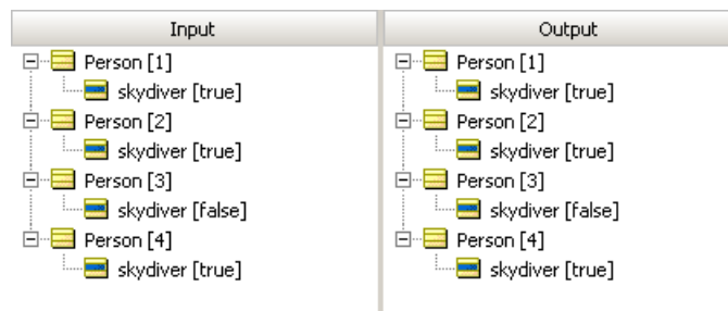
Figure 160: Ruletest with 3 Skydivers
