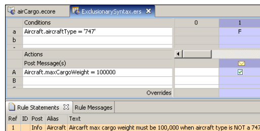
Figure 67: Exclusionary Logic Using Negated Value
