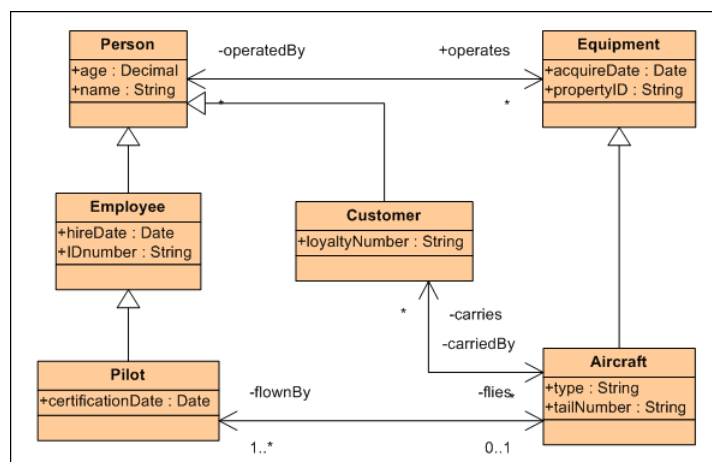
Figure 29: Rose UML Model Showing Inheritance
