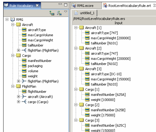
Figure 45: Test the Rule Using “Root-Level” Vocabulary Terms
