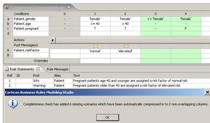
Figure 199: Example after Completeness Check
