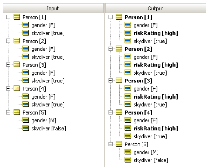
Figure 167: Ruletest
