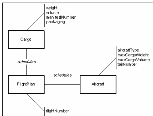
Figure 40: Fact Model
