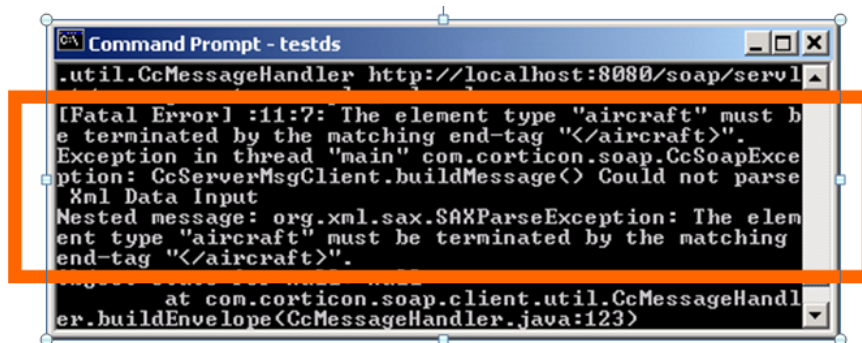
Figure 234: Server Window Message Highlighting Incorrect SOAP Request Structure
