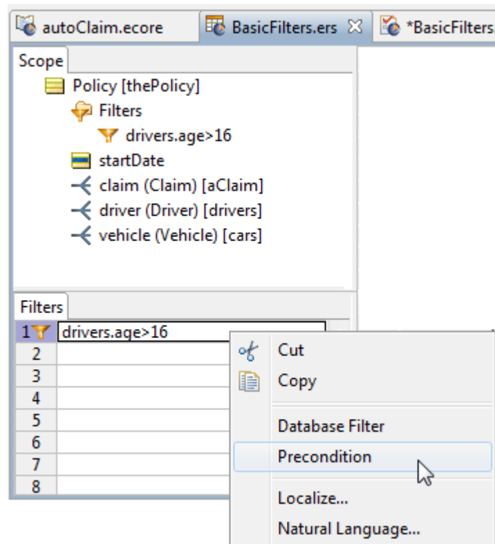
Figure 151: Selecting Precondition Behavior from the Filter Right-Click Popup Menu
