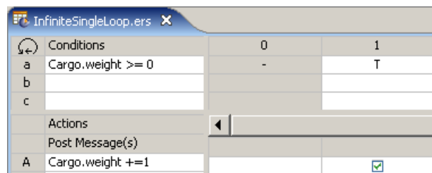
Figure 117: Example of an Infinite Single-Rule Loop
