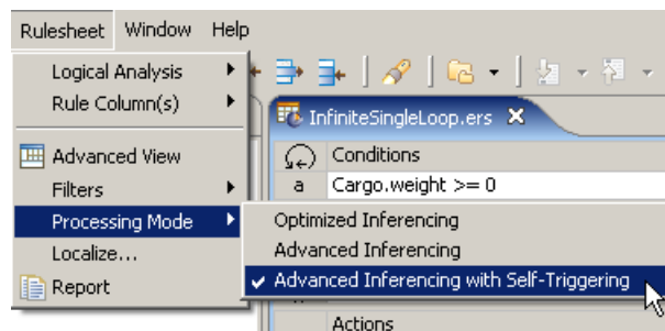
Figure 116: Selecting Advanced Inferencing with Self-Triggering Processing Mode for a Rulesheet
