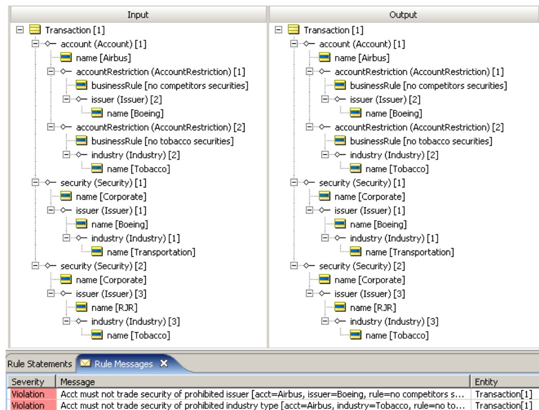
Figure 172: Ruletest
