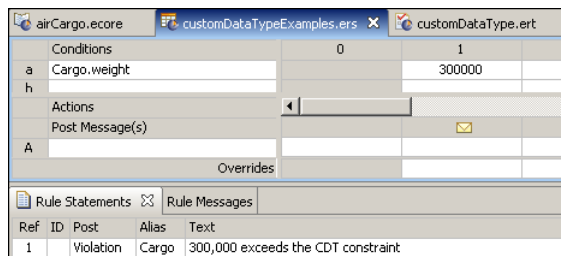
Figure 7: Using Custom Data Types in a Rulesheet
