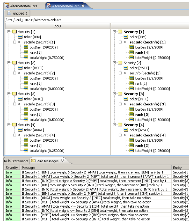
Figure 84: Rulesheet for Alternate Security Ranking Model Rules
