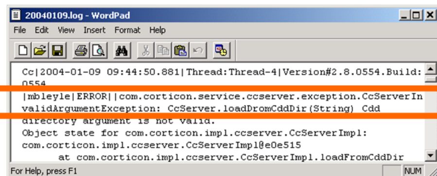
Figure 241: Log Excerpt Highlighting Missing \cdd Directory
