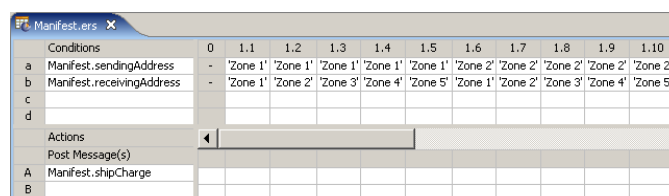
Figure 205: Rule 1 Expanded to Show Sub-Rules
