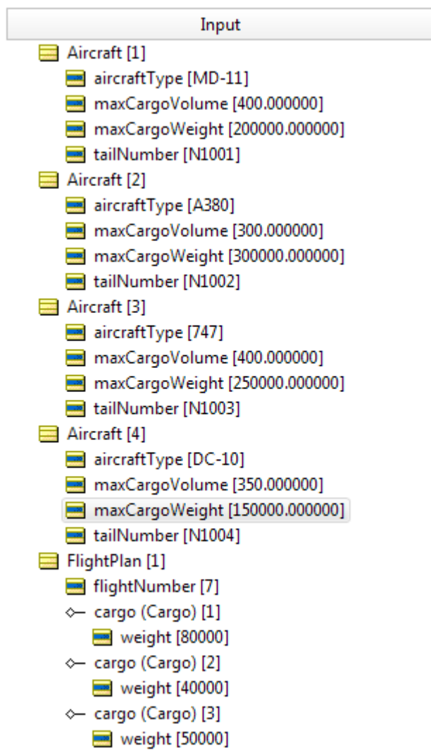
Figure 175: Sample Input Ruletest
