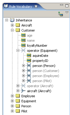
Figure 31: Vocabulary with Inheritance
