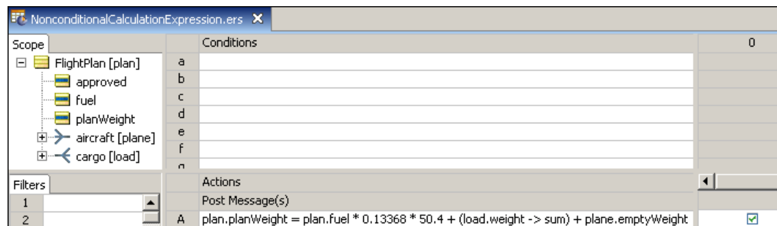
Figure 107: A Calculation in a Nonconditional Expression
