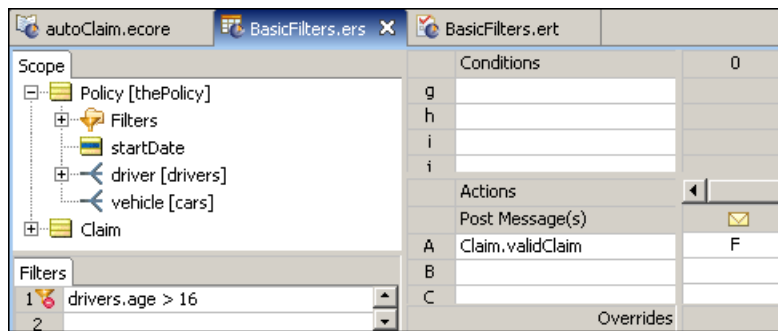
Figure 153: Rulesheet with a Filter in Precondition Mode
