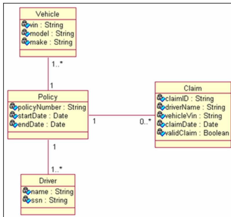
Figure 92: UML Class Diagram
