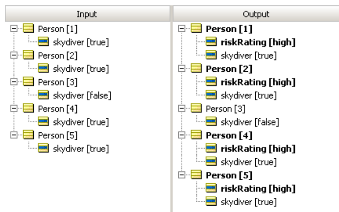
Figure 161: Ruletest with 4 Skydivers
