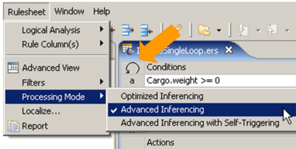
Figure 114: Selecting Advanced Inferencing Processing Mode for a Rulesheet
