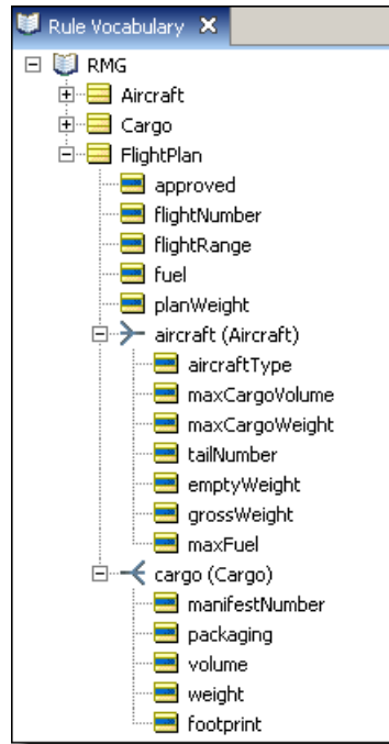
Figure 105: Basic Tutorial Vocabulary Extended
