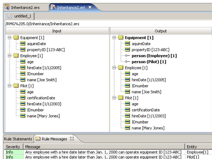
Figure 38: Inheriting an Association
