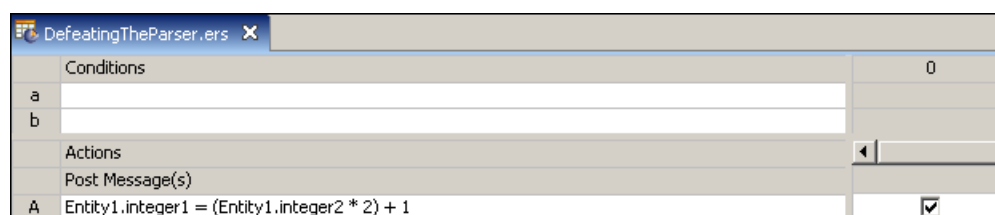
Figure 102: LHS and RHS Resolve to Integers
