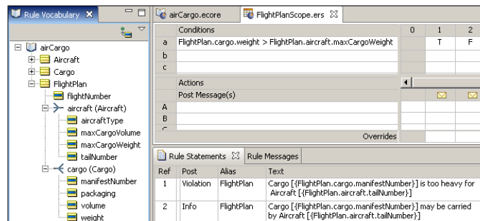
Figure 48: Rule Expressed Using FlightPlan as the Rule Scope
