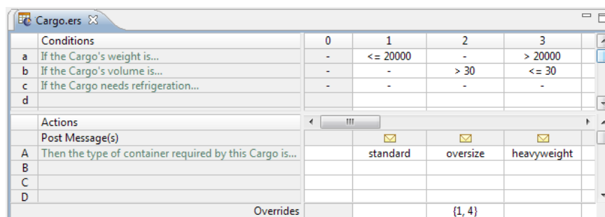
Figure 227: Rulesheet with natural language text
