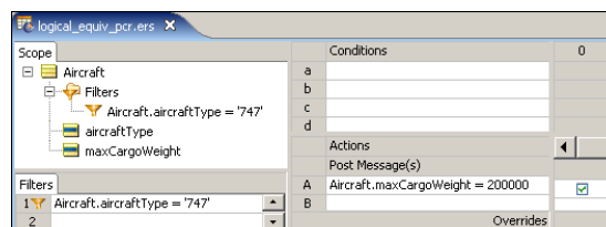
Figure 62: Rulesheet Using a Filter and Nonconditional Rule
