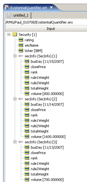
Figure 90: Ruletest for Testing exists Condition Rules
