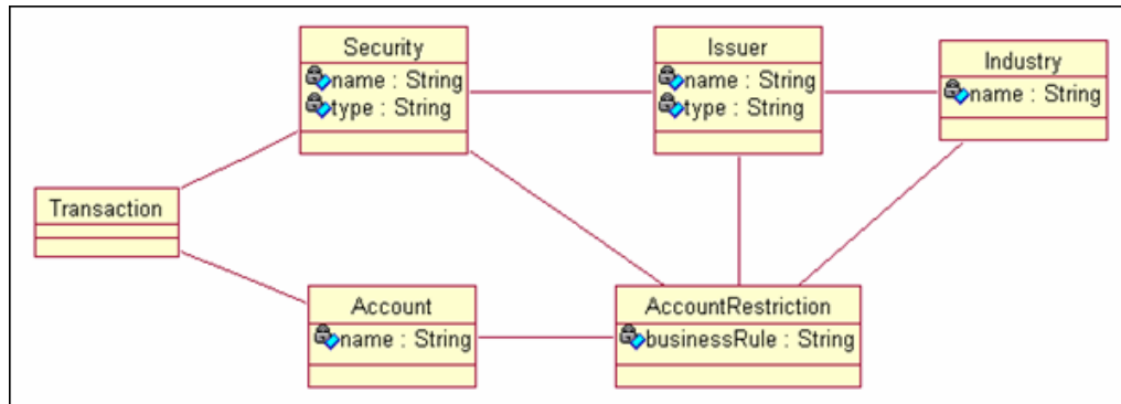
Figure 170: UML Class Diagram of Sample Vocabulary
