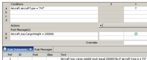
Figure 63: Rulesheet Using a Conditional Rule
