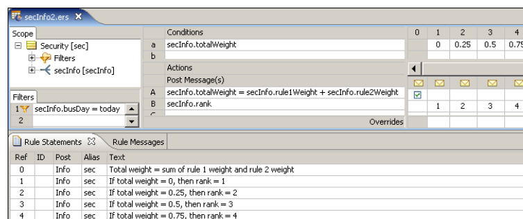
Figure 79: Rulesheet with Total Weight Calculation and Rank Determination
