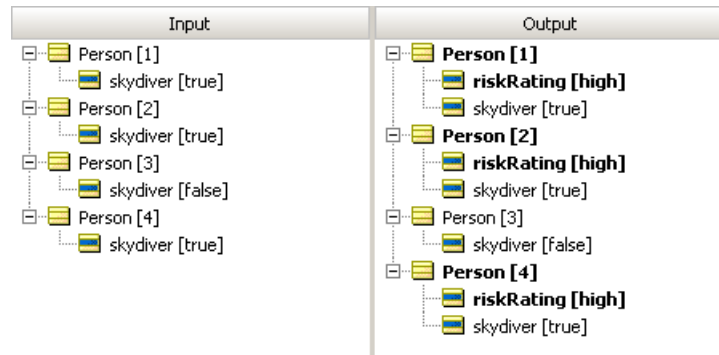
Figure 162: Ruletest with 3 Skydivers
