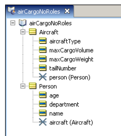
Figure 54: Vocabulary without Roles
