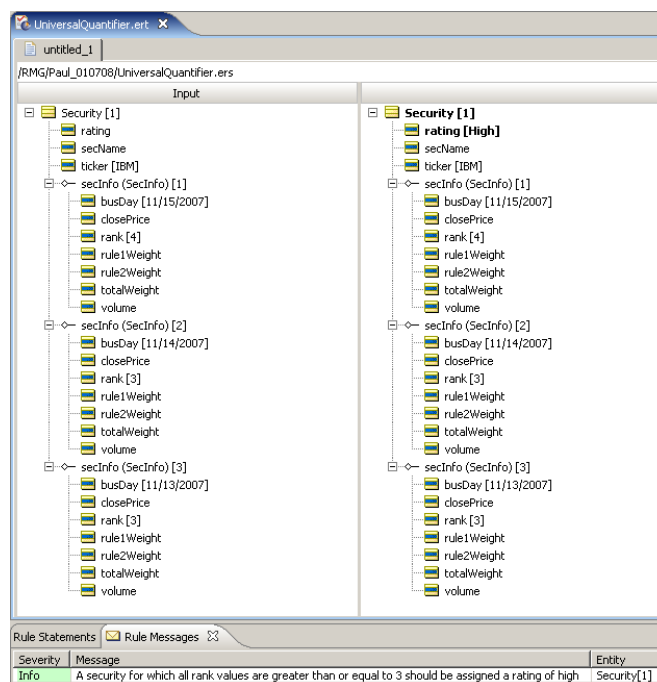
Figure 88: Ruletest for “for all” Condition Rules
