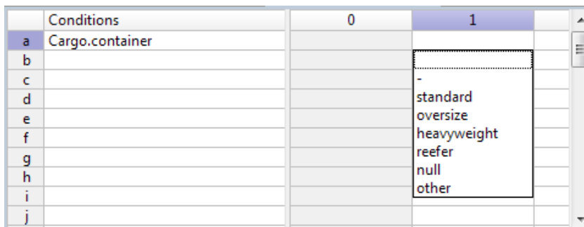
Figure 22: Using Custom Data Types in the Rulesheet
