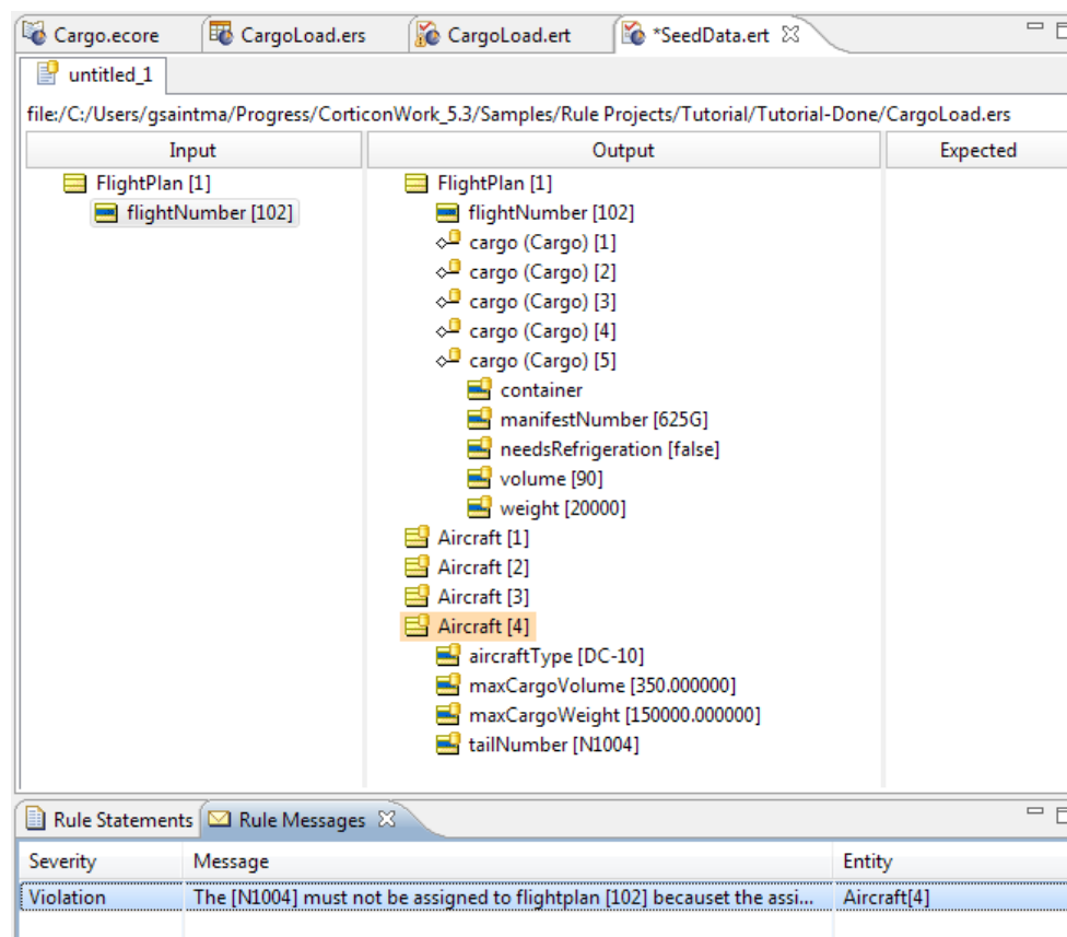
Figure 181: Results Ruletest Showing a Successful Extend-to-Database Retrieval
