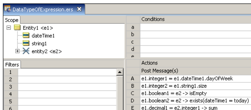
Figure 101: Examples of Expression Datatypes
