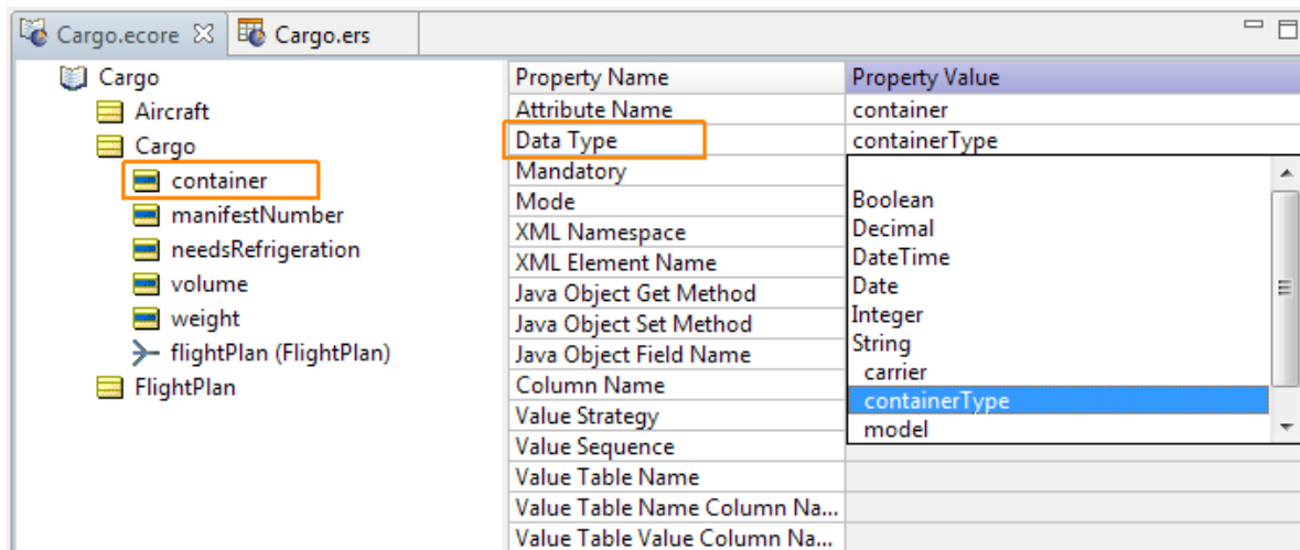
Figure 21: Using Custom Data Types in the Vocabulary
