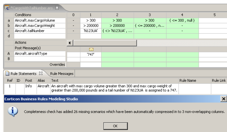
Figure 213: Remaining Columns Produced by the Completeness Checker
