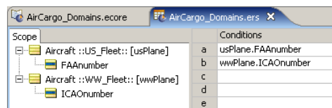
Figure 27: Non-unique Entity names after defining Aliases
