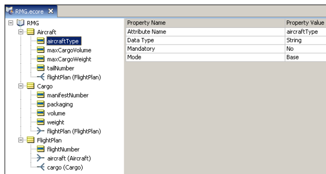
Figure 4: Vocabulary Window in Corticon Studio
