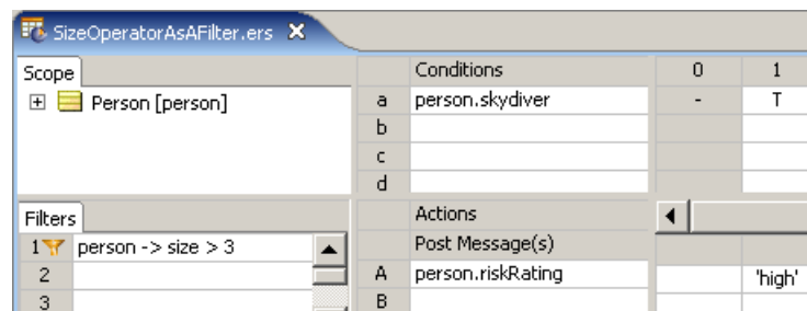
Figure 159: Collection Operator in Filter row
