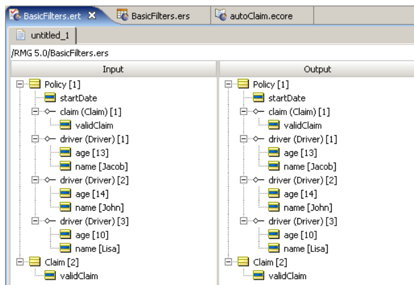
Figure 154: Testsheet for a Filter in Precondition Mode
