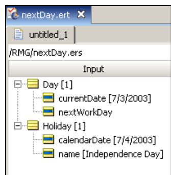
Figure 131: Ruletest for Holiday Rules
