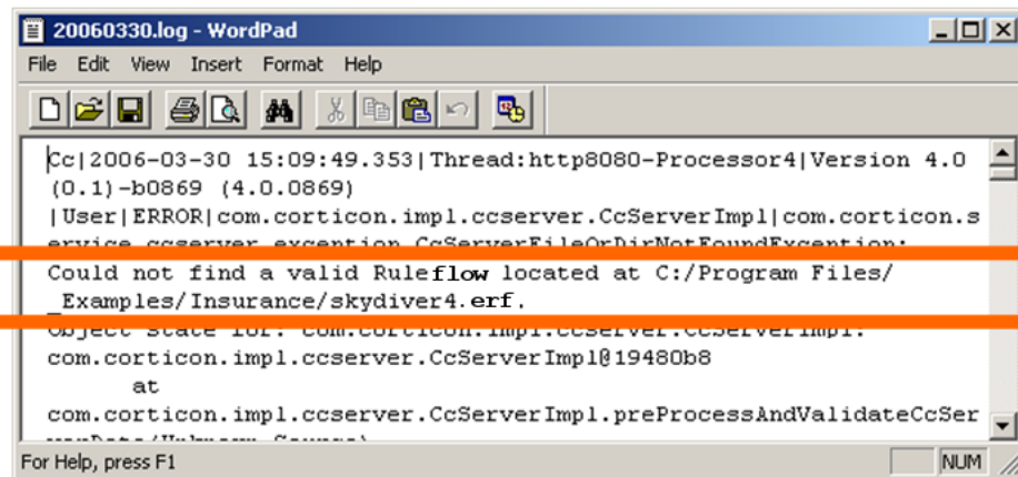
Figure 239: Log Excerpt Highlighting Incorrect .erf Path
