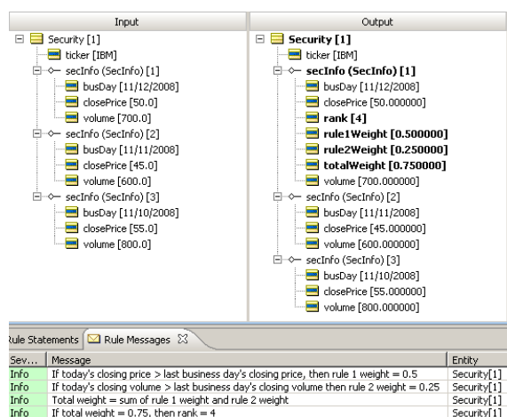
Figure 81: Ruletest for Security Ranking Model Rules
