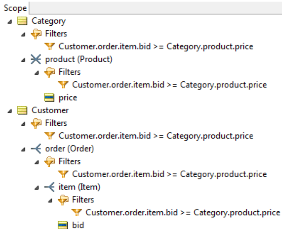
Figure 144: Application of the filter to the Scope's tree structure
