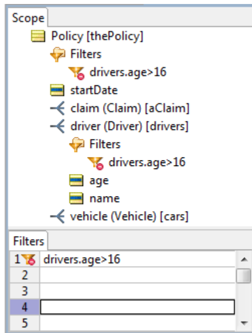
Figure 152: A Filter in Precondition Mode
