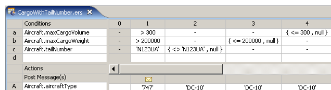
Figure 215: Missing Rules with Actions Assigned
