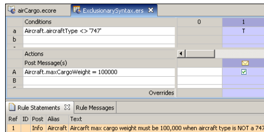
Figure 66: Exclusionary Logic Using Boolean Condition, Pt. 2
