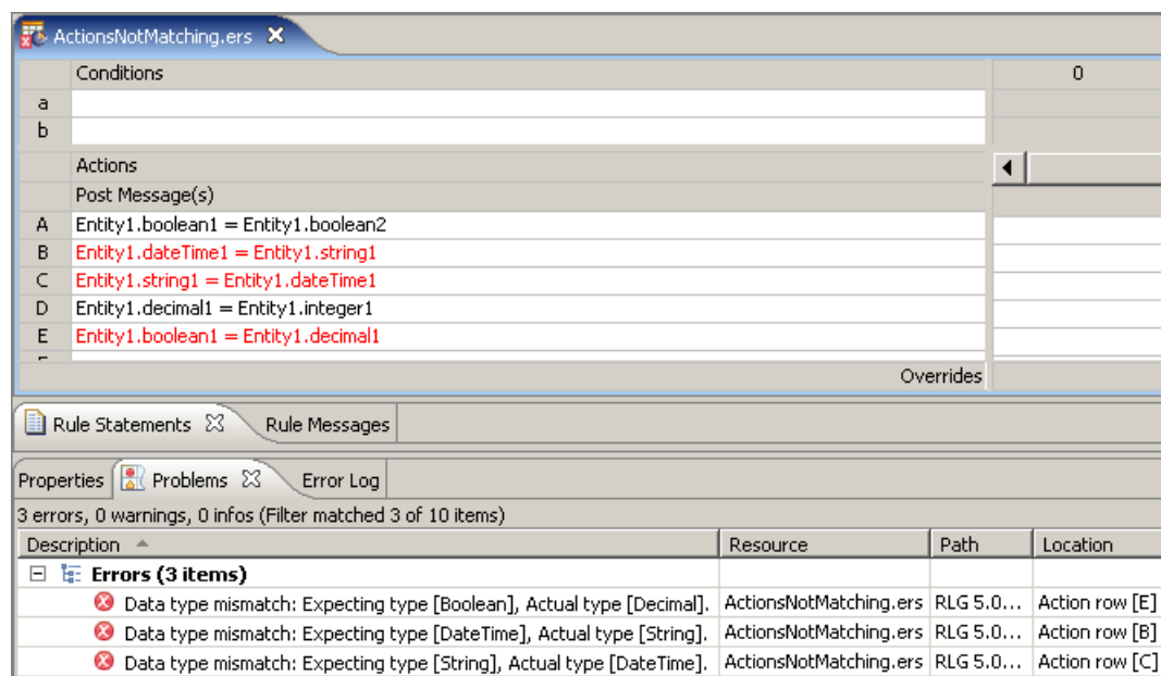
Figure 99: Datatype Mismatches in Assignment Expressions
