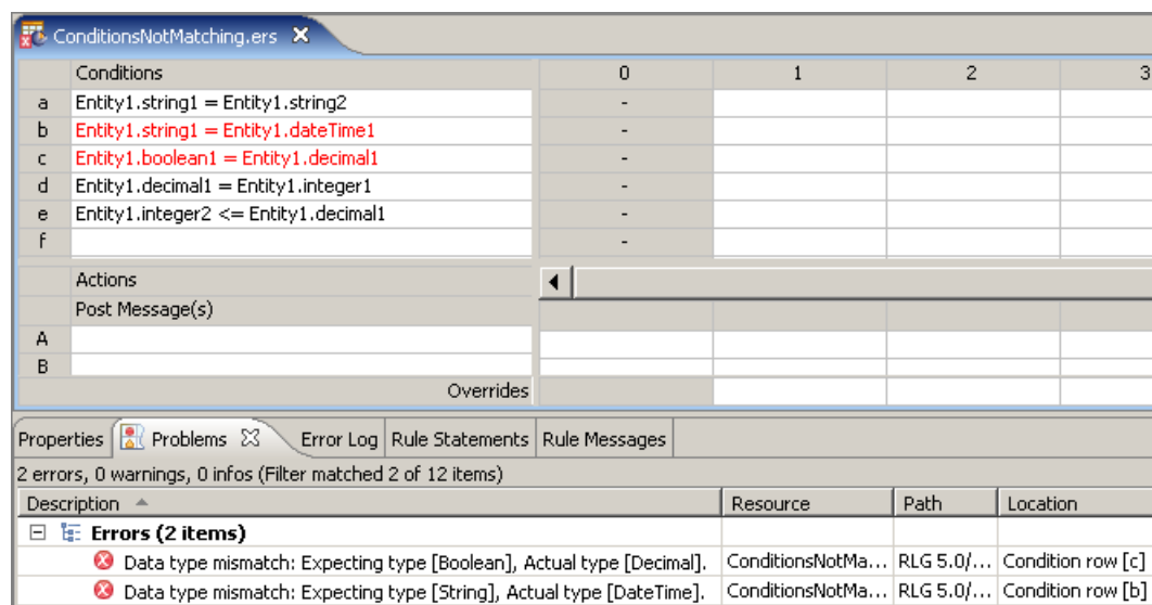
Figure 100: Datatype Mismatches in Comparision Expressions
