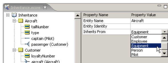
Figure 30: Selecting Ancestor Entity for Descendant
