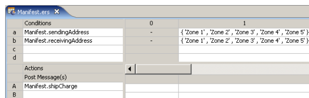
Figure 204: Rulesheet with Conditions Automatically Populated
