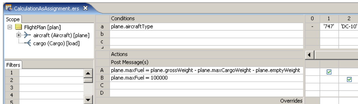
Figure 110: A Calculation in an Action Expression
