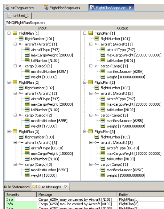
Figure 50: Ruletest Results Using Scope – Note no Violations
