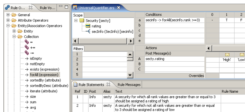
Figure 86: Rulesheet with Universal Quantifier (“for all”) Condition
