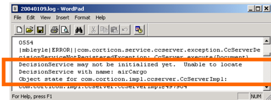
Figure 240: Log Excerpt Highlighting Unknown Decision Service Name
