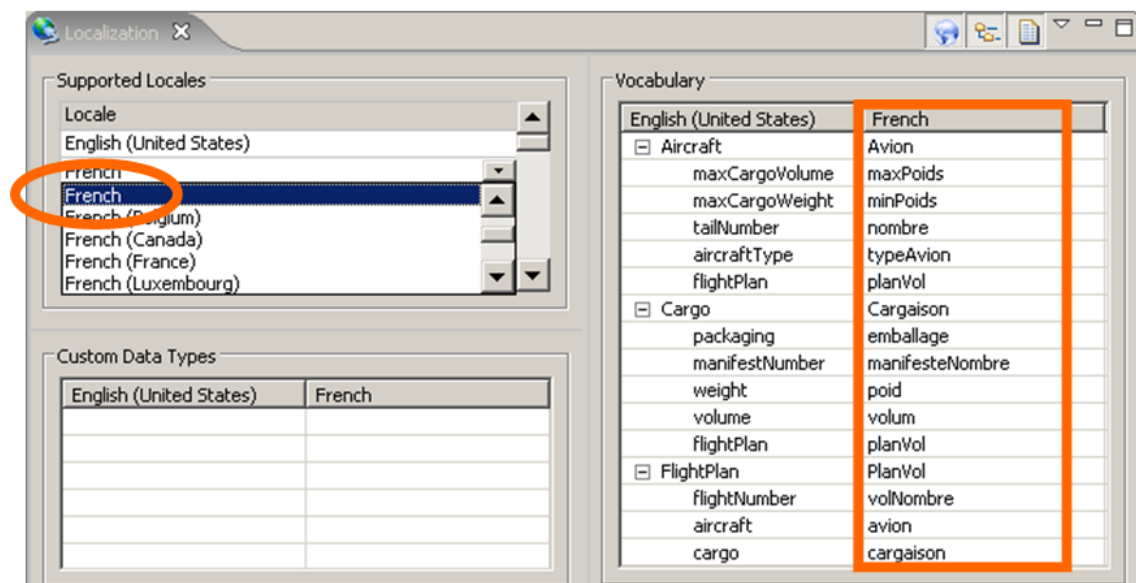
Figure 221: Selecting and populating a second locale
