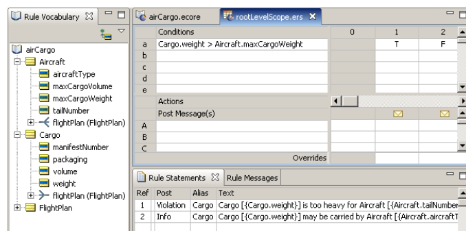
Figure 41: Expressing the Rule Using “Root-Level” Vocabulary Terms
