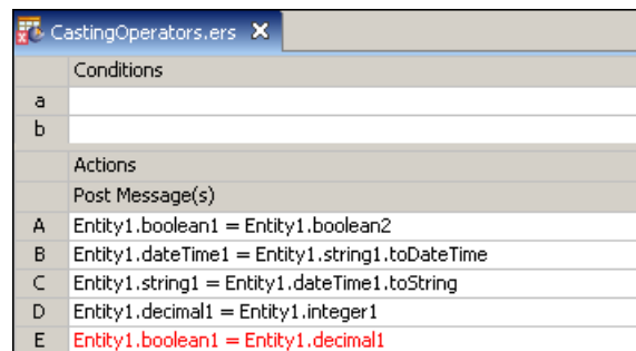
Figure 104: Using Casting Operators
