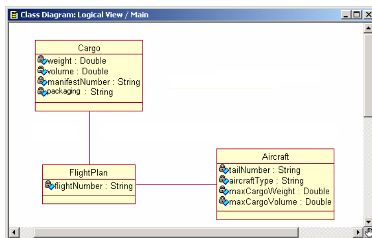
Figure 3: UML Class Diagram
