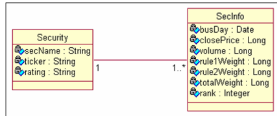
Figure 76: Security Vocabulary UML Class Diagram
