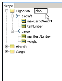
Figure 51: Defining an Alias in the Scope window
