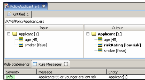
Figure 184: Ruletest
