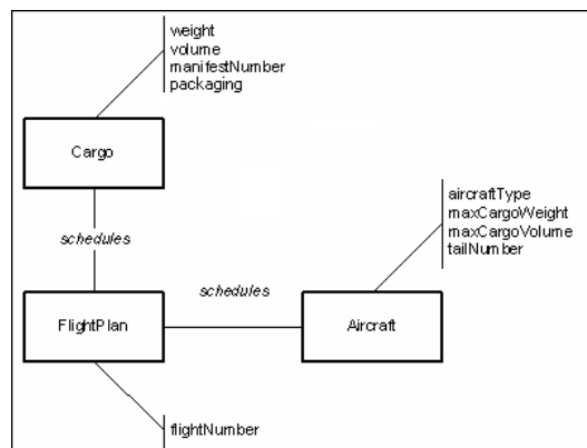
Figure 2: Fact Model
