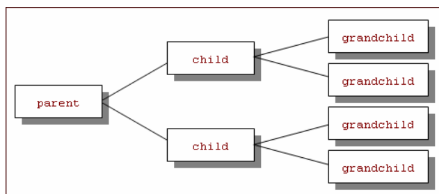
Figure 75: 3-Level Collection
