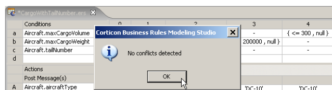
Figure 216: Proof that no New Conflicts have been Introduced by the Completeness Check
