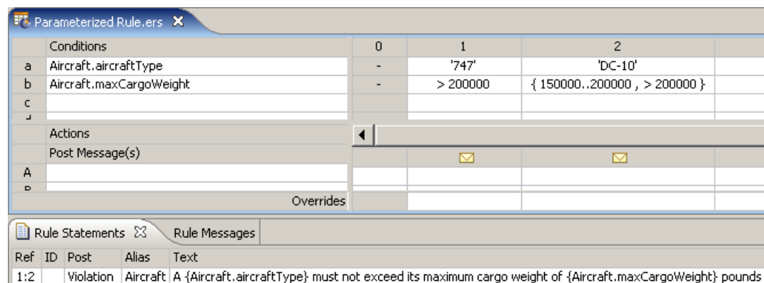
Figure 169: Parameterized Rules
