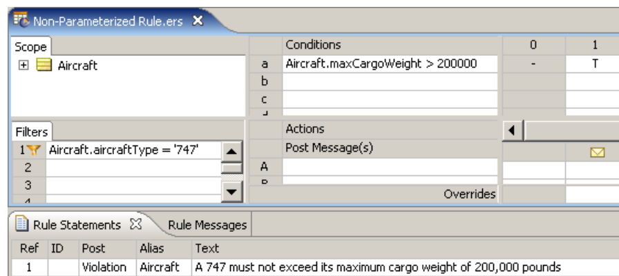
Figure 168: Non-Parameterized Rule
