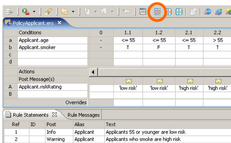
Figure 192: Expanding Rules to Reveal Components
