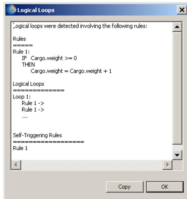
Figure 125: A Single-Rule Loop Detected by the Check for Logical Loops Tool
