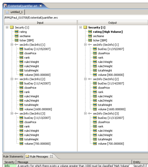
Figure 91: Ruletest for exists Condition Rules
