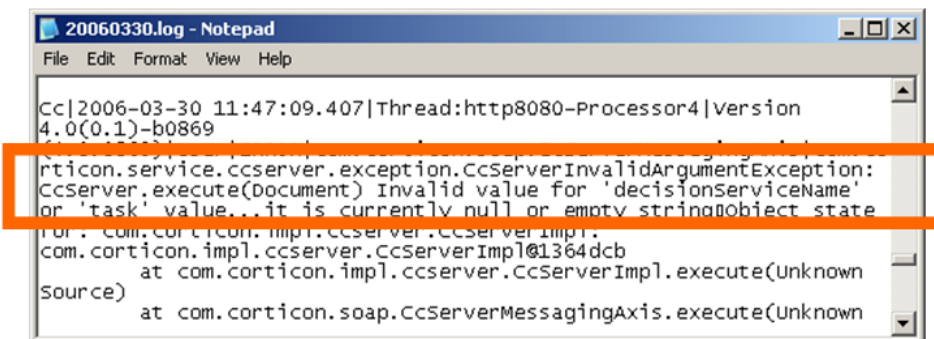
Figure 235: Log Excerpt Highlighting Missing Decision Service Name in SOAP Request
