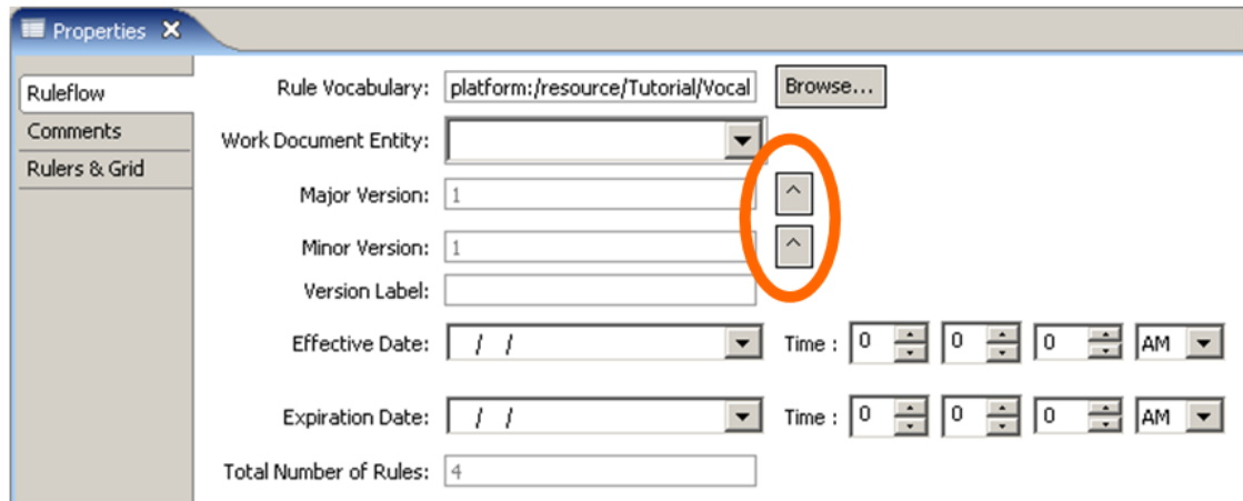
Figure 218: Assigning a Version Number to a Ruleflow
