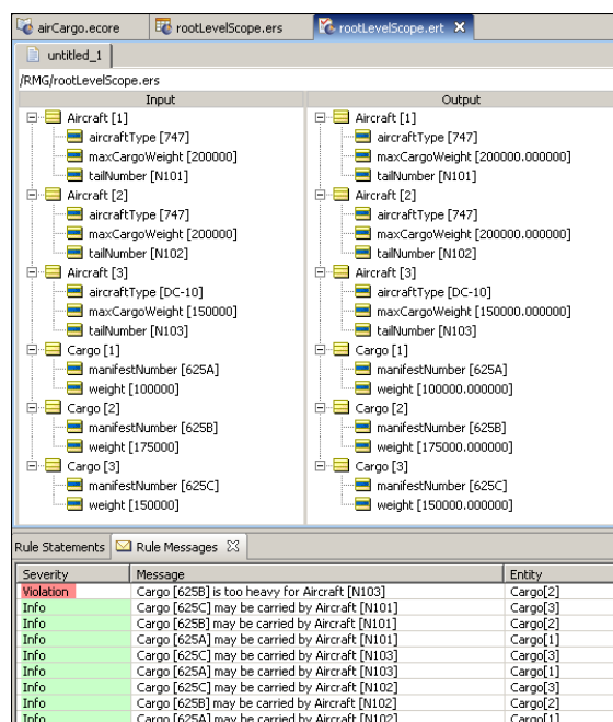
Figure 46: Results of the Ruletest
