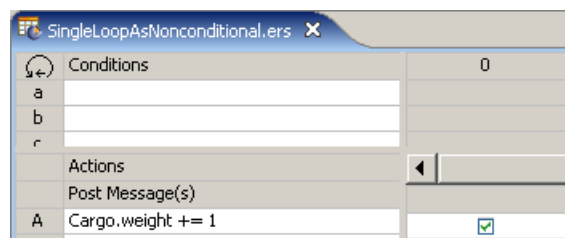
Figure 118: Example of an Infinite Loop created by a Self-Triggering Rule
