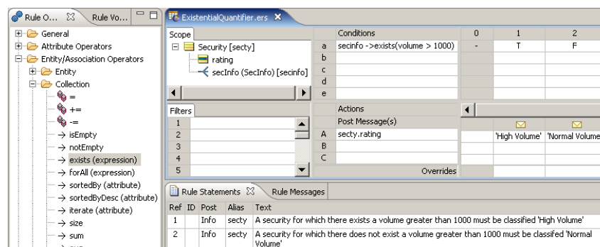
Figure 89: Rulesheet with Existential Quantifier (“exists”) Condition
