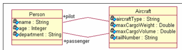
Figure 55: UML Class Diagram with Roles
